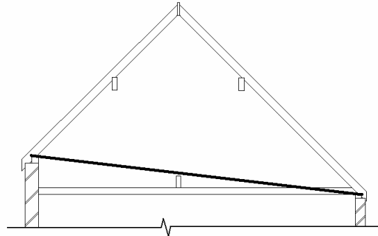
diagram 1. (Roof Section)
